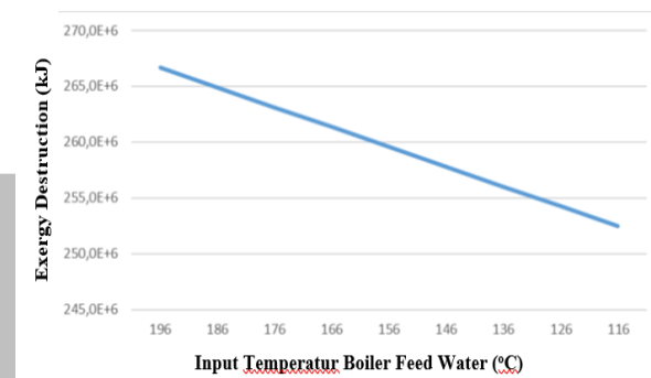
Figure 4.2. Temperature BFW Reduction versus Exergy Destruction
