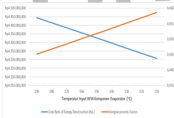
Figure 4.3. BFW Temp Reduction against Cost rate of Exergy Destruction ( \dot{C}_{D,k} ) and Exergoeconomic Factor ( f_k ) Chart
