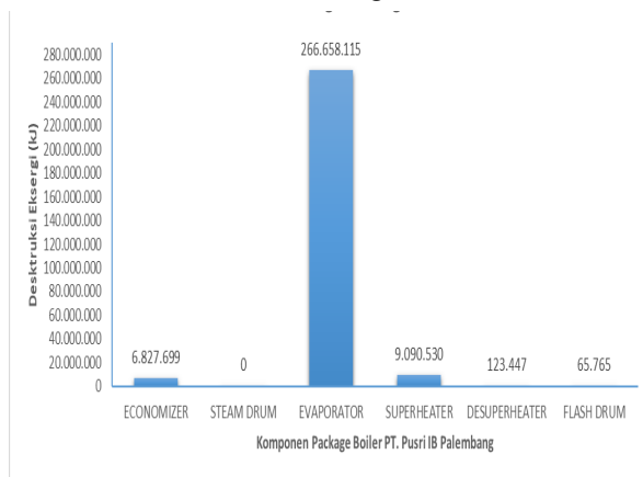
Figure 4.1. Exergy Destruction Chart of Package Boiler
